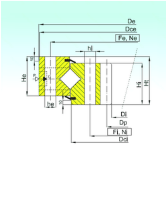
ZR1.40.1385.400-1SPPN Bearing 2D drawings and 3D CAD models
