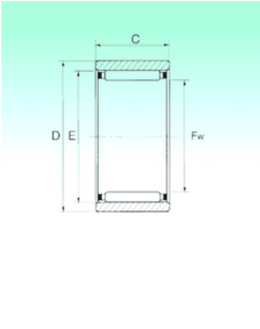
RNAO 17x25x13 Bearing 2D drawings and 3D CAD models
